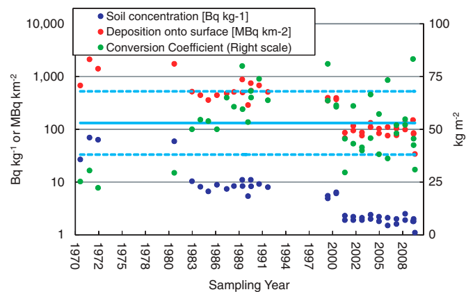
Fig. S5. Relationship between ^{137}\text{Cs} deposition and concentration in soil for determining conversion coefficient (CC). The historical observed data were obtained from the environmental radiation database (1) maintained by the Japan Chemical Analysis Center. The observed data at the same location and on the same day in different units of \text{Bq kg}^{-1} (top 5 cm soil) and \text{MBq km}^{-2} ( \text{Bq m}^{-2} ) are assumed to be the same sample and used the data for calculating the CC ( \text{kg m}^{-2} ). Solid and dotted lines denote mean CC value and its standard deviations, respectively.
