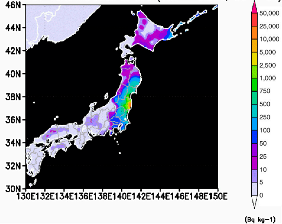
Movie S4. Estimated ^{137}\text{Cs} concentration range in soil using DRT of 0.001 and conversion coefficient (CC) of 38, 53, and 68 \text{ kg m}^{-2} over Japan. CCs of 38, 53, and 68 \text{ kg m}^{-2} correspond to -1\sigma , mean value, and +1\sigma in Fig. S5, respectively. Outputs 0.2^\circ \times 0.2^\circ were interpolated into finer resolution using cubic interpolation. The Merged IBCAO/ETOPO5 Global Topographic Data Product (1) was used to mask out ocean area below 0 m above sea level (a.s.l.).
