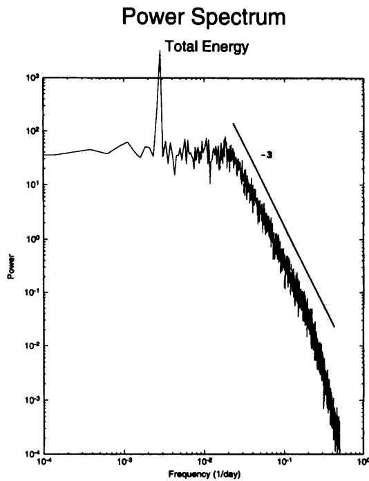
Fig. 4. As in Fig. 2, but for the experiment with the annual cycle forcing for the 100-year integration. The power spectrum is estimated by the FFT routines and is smoothed by averaging 8 terms of the original power spectrum. The sharp spectral peak corresponds to the annual cycle.
