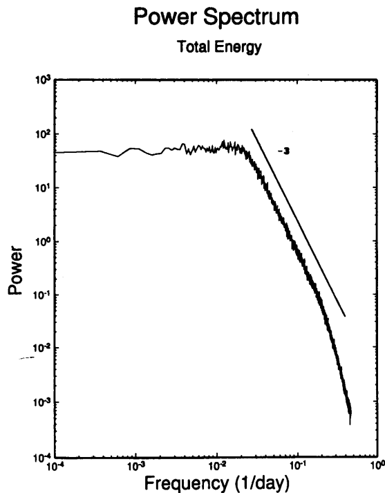
Fig. 2. Power spectrum of the time series of the total energy for the 1000-year integration. The power spectrum is estimated by the FFT routines and is smoothed by averaging 64 terms of the original power spectrum.
