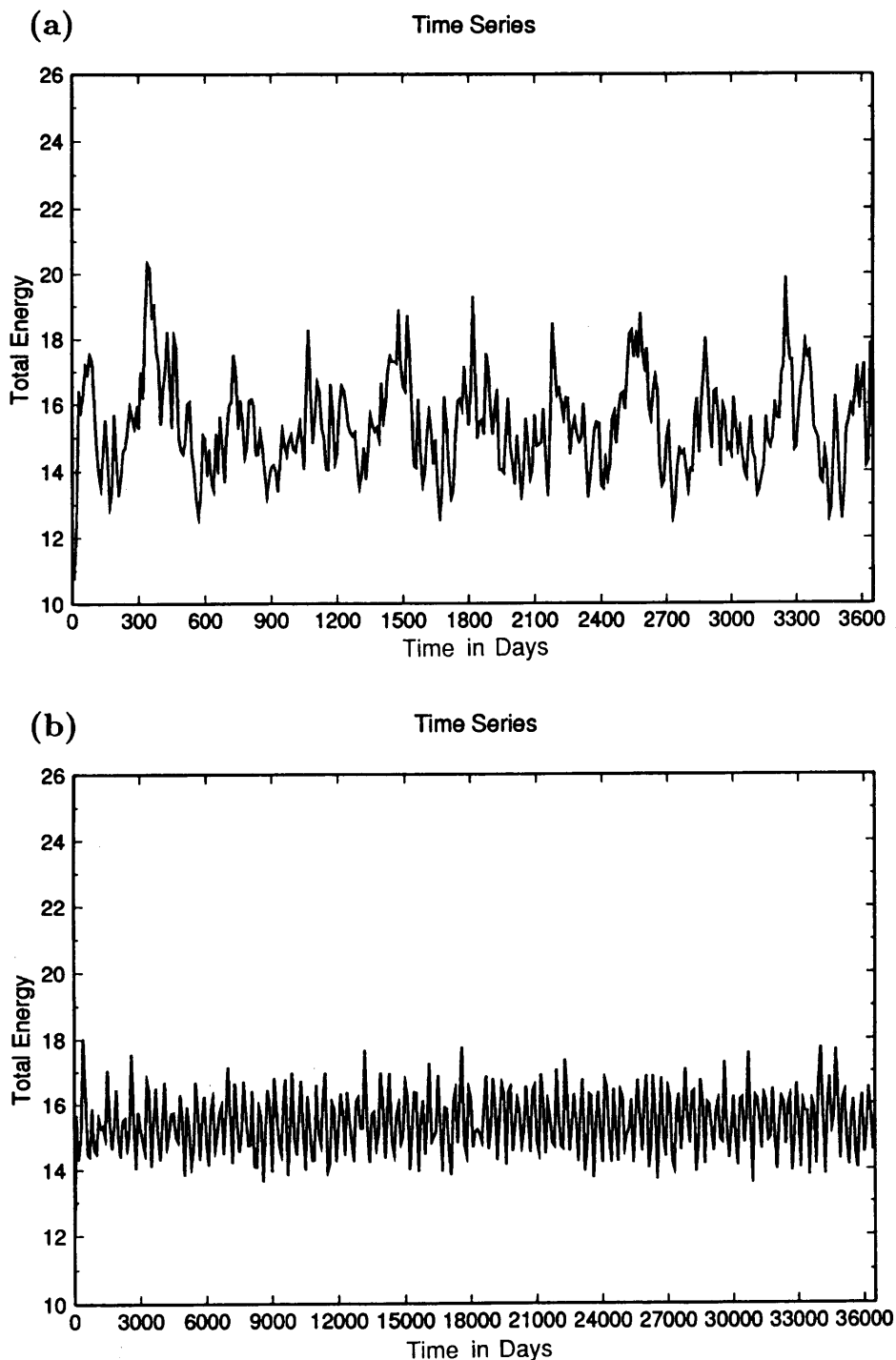
Fig. 3. As in Fig. 1, but for the experiment with the annual cycle forcing. The values in the figures contain 365 points of data for (a) 10-day mean during 10 years and (b) 100-day mean during 100 years, respectively. The units are 10^5 \text{ Jm}^{-2} .
