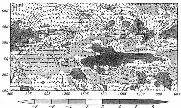
図11 図10と同様, ただしデータは ECMWF Fig. 11 Same as in Fig. 10 but for ECMWF data.
