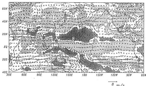
b) Strong Monsoon Season 84,85,90
