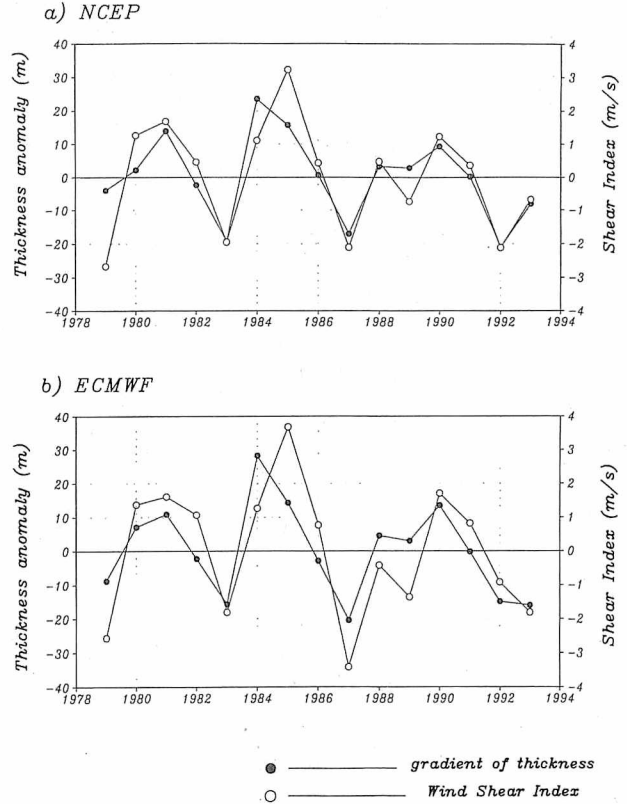
図9 夏季(6月-9月)平均モンスーン強度インデックスの経年変動 a) NCEP b) ECMWF, 黒丸は Kawamura (1998) に基づく対流圏上層(200hPa-500hPa)の層厚の南北差(20°Nを境界とした海域と陸域の差), 白丸は Webster and Yang (1992) に基づくモンスーン領域の東西風鉛直シア。 Fig. 9 a) Interannual variations for the mean summer (Jun-Sep) monsoon index using NCEP data. The monsoon index is defined as the meridional difference in area averaged upper-tropospheric (200hPa-500hPa) thickness, based on Kawamura (1998), and as the area averaged vertical shear of zonal wind based on Webster and Yang(1992). b) Same as a) but for ECMWF data.
