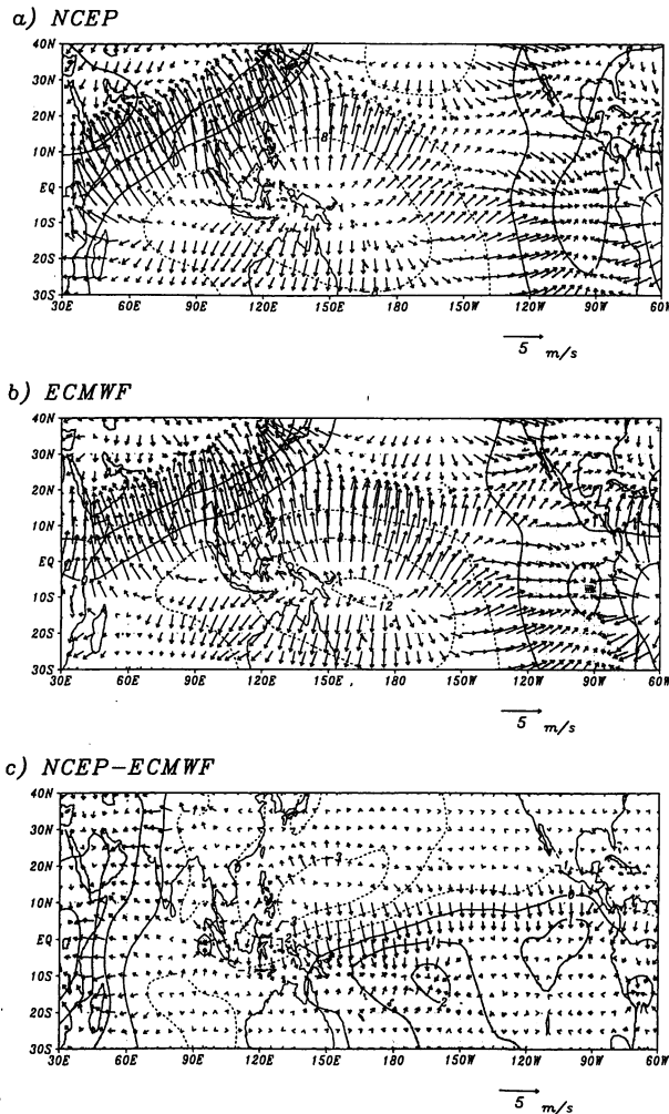
図3 図1と同様な期間での200 hPa面の速度ポテンシャルと発散風 等値線間隔は a), b) 4 \times 10^6 (m^2/s) , c) 1 \times 10^6 (m^2/s) Fig.3 Same period as for Fig.1 but for a 200 hPa velocity potential and divergent wind field. The contour interval is 4 \times 10^6 (m^2/s) in a), b) and 1 \times 10^6 (m^2/s) in c).
